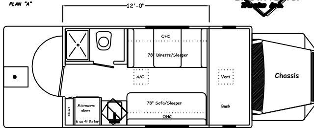
12' REAR DOOR PLAN "A"
