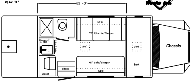
12' SIDE DOOR PLAN "A"
