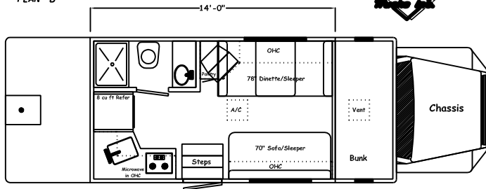
14' SIDE ENTRANCE PLAN "B"
